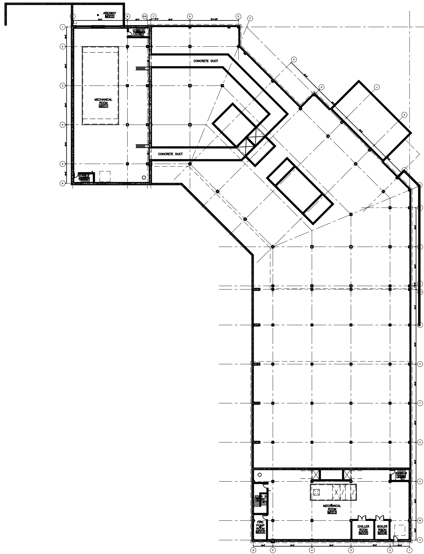
MECHANICAL LEVEL (M1) FLOOR PLAN
